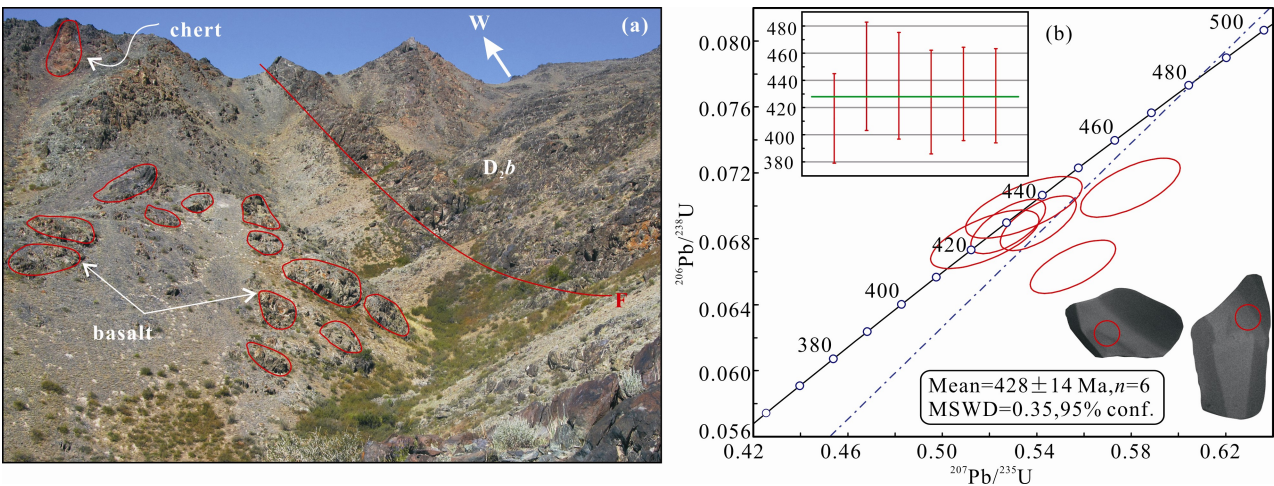
Fig. 1. Field photographs of typical outcrop (a), U-Pb concordia diagram of zircon grains for the basalts (b) within the Hatu tectonic mélange in southern West Junggar
