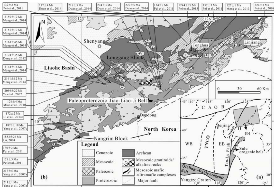
Fig. 1. Geological sketch map of the Liaodong Peninsula and adjacent regions. (a) Subdivision of the NCC and surrounding area; (b) Geological map of the Liaodong Peninsula and adjacent regions emphasizing the distribution of mafic rocks and their ages.
