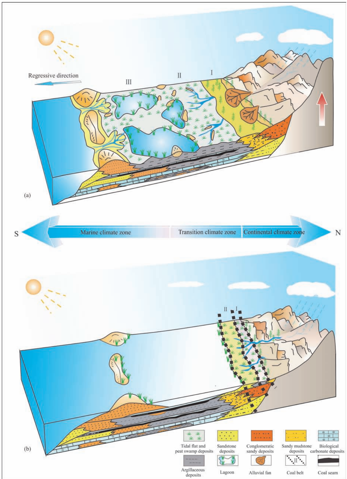
Fig. 4. Coal-forming paleogeographic model and the coal-forming belt distributions during different time periods of regression and transgression in the Carboniferous-Permian epicontinental sea basins of northern China.
