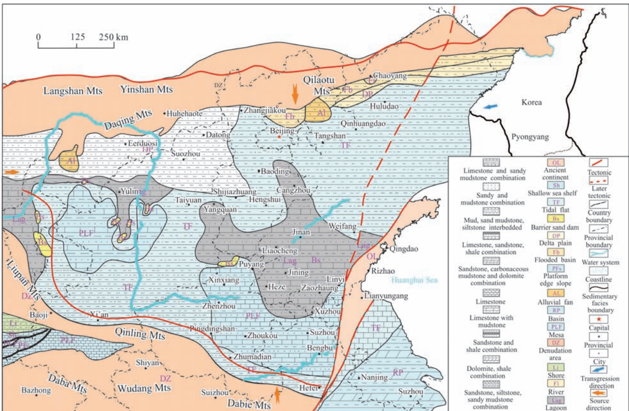
Fig. 3. Coal-forming paleogeography during the Early Permian Period in North China.
